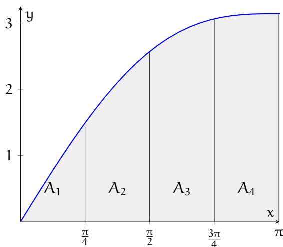
Figure 4.4: f(x) = \sin x + x divided into 4 regions
