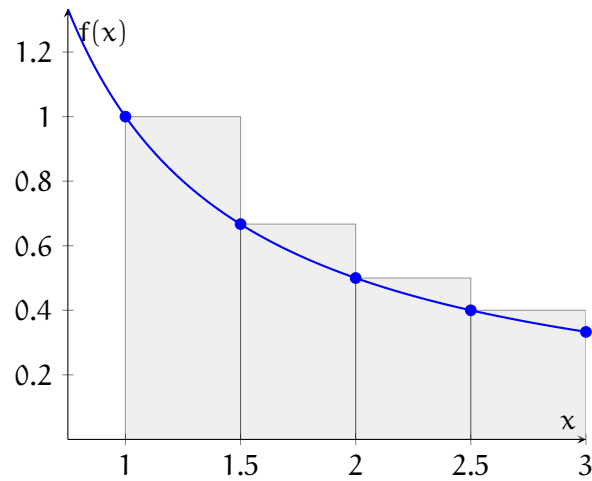
Figure 4.11: L_4 for f(x) = \frac{1}{x}
