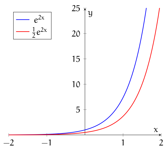
Figure 3.6: e^{2x} and its antiderivative \frac{1}{2}e^{2x}
