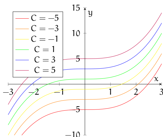
Figure 3.4: If F'(x) = x^2 , then the general solution is F(x) = \frac{1}{3}x^3 + C
