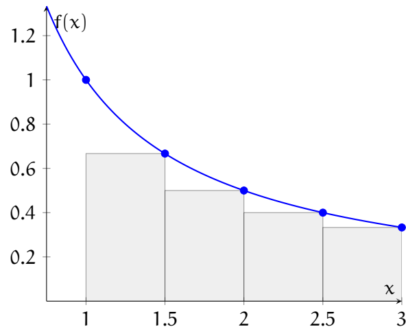
Figure 4.10: R_4 for f(x) = \frac{1}{x}
