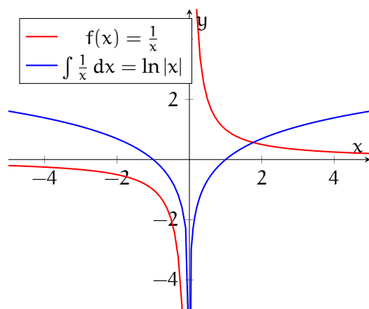
Figure 3.5: \frac{1}{x} and its antiderivative, \ln|x|
