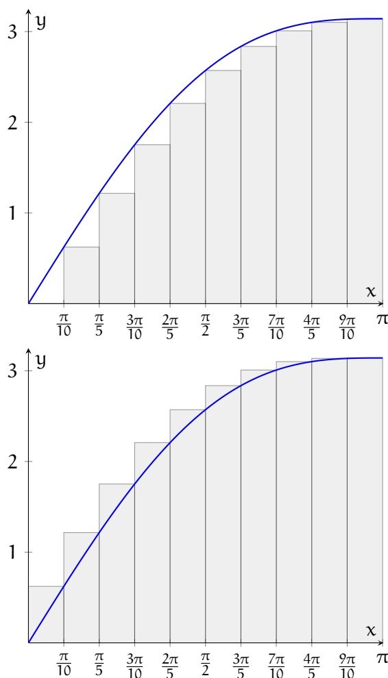
Figure 4.7: \sin x + x broken into 10 intervals using either the left or right value to determine the height.
