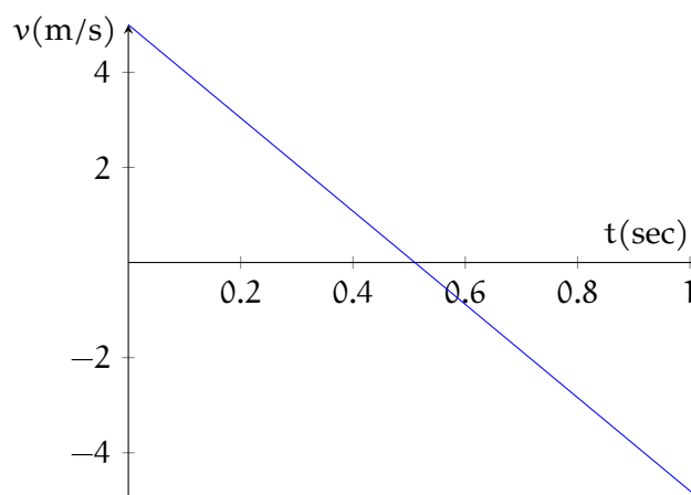
Figure 4.1: Velocity of a hammer thrown upwards at 5 m/s
