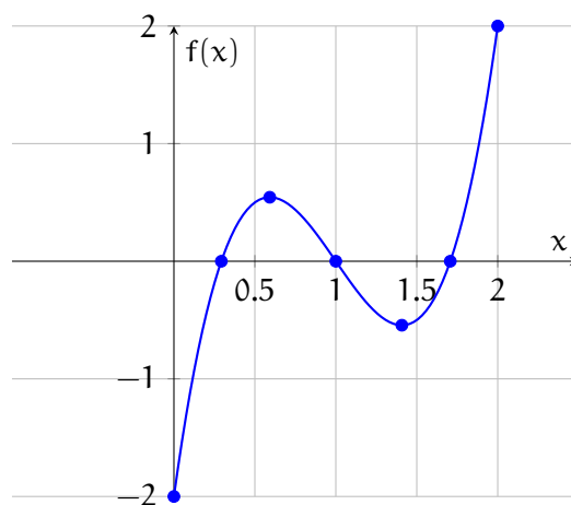
Figure 3.1: Plot of f with select points
