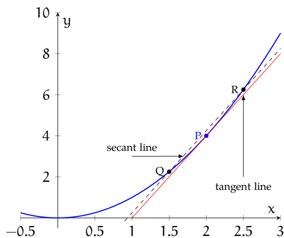
Figure 2.2: The slope of the secant line is approximately the slope of the tangent line
