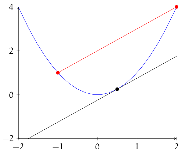
Figure 2.8: f(x) = x^2
